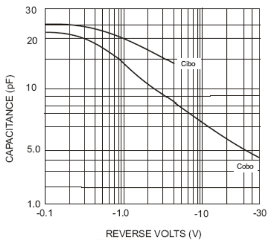
Fig. 6, Typical Capacitance
